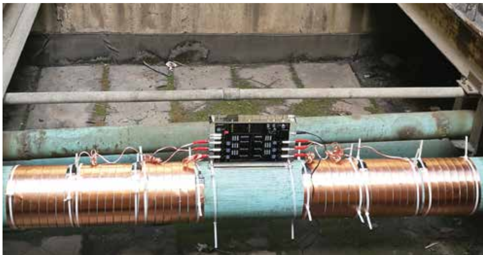
Vulcan S100 was installed on the inlet water main of cooling tower in Huaneng Dalian power plant. The pipe diameter is 150 mm and the material is steel.
